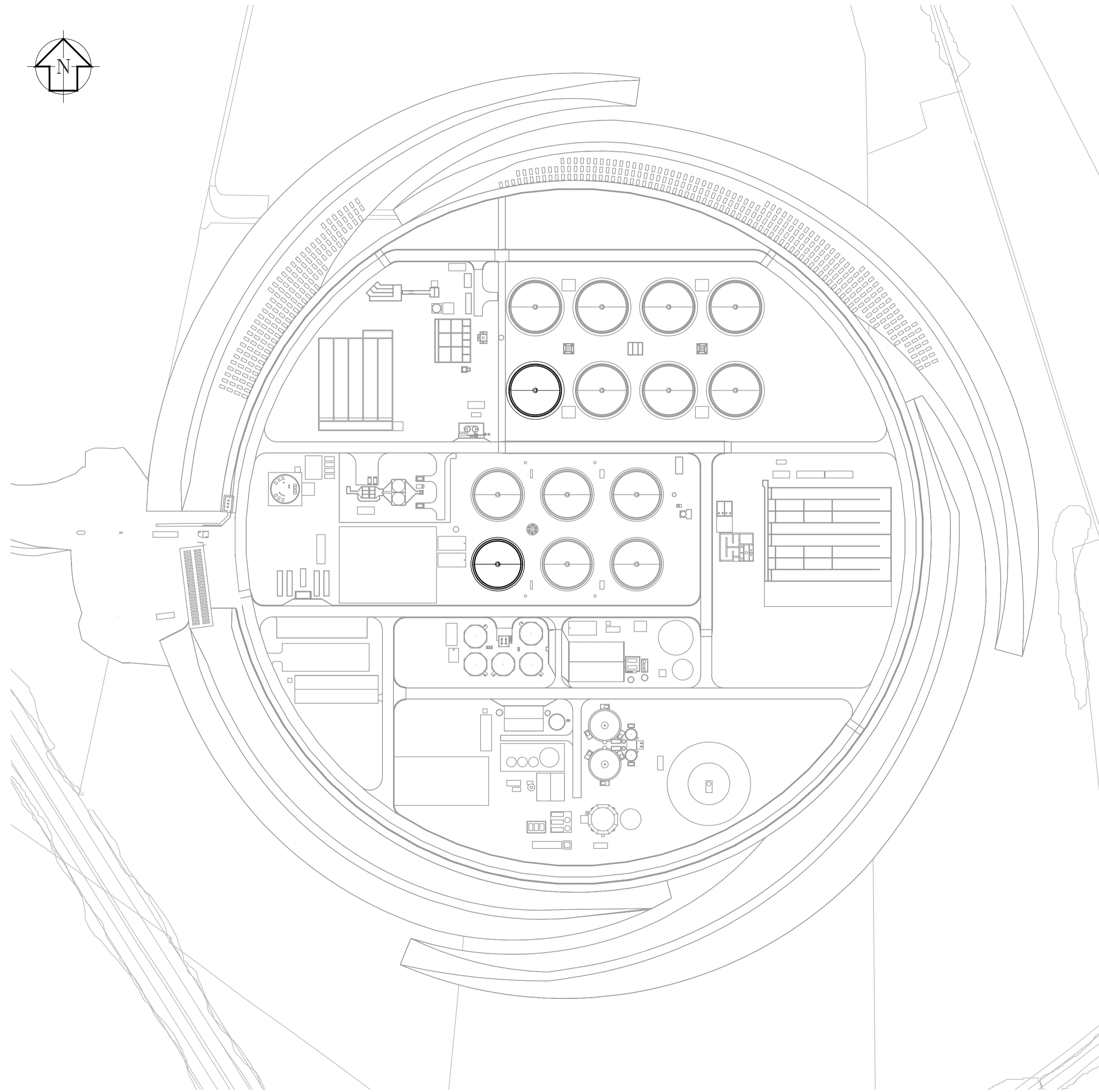
EXTENSION (SECOND PHASE)
